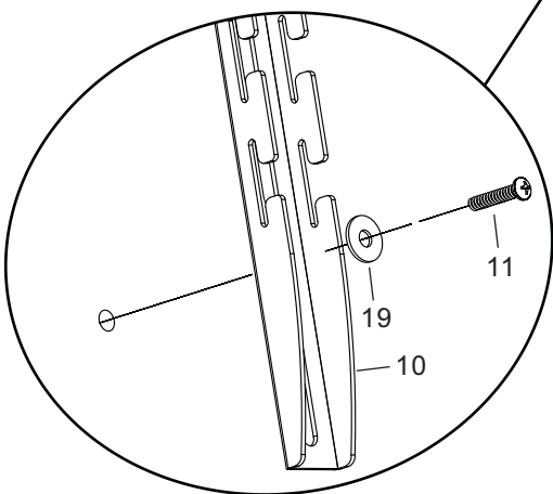
M5 Diameter Bolt
