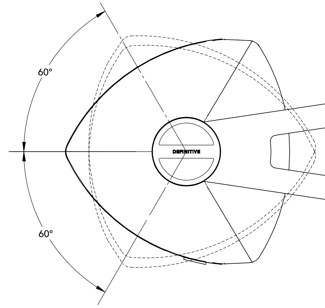
MAXIMUM ROTATION
